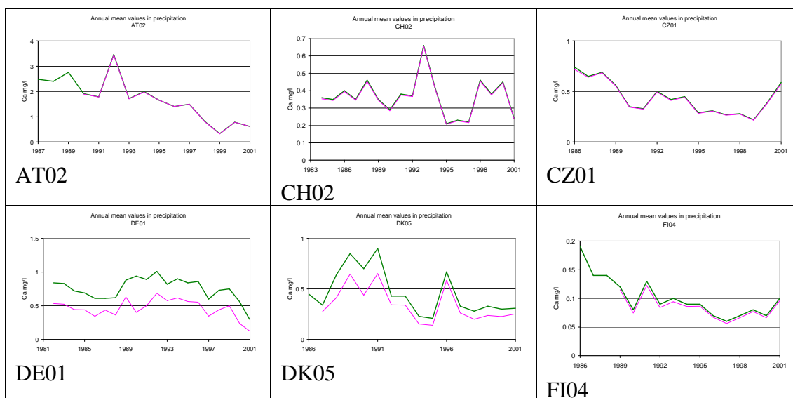
Figure BC-1 Calcium in precipitation (mg/l) at a number of EMEP sites all over Europe.
