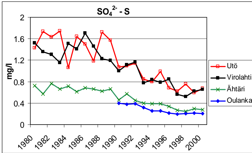
Figure 14. Annual mean concentrations of sulphate in precipitation.
