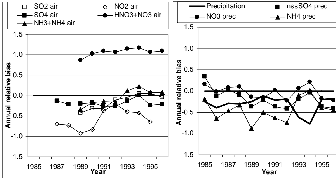
Figure 17 a. The annual relative bias of the modelled atmospheric concentrations in 1985–1996 averaged over Virolahti, Ähtäri and Oulanka.
