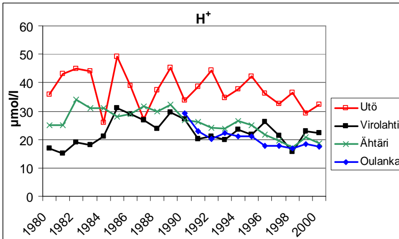
Figure 15. Annual mean concentrations of the hydrogen ion.
