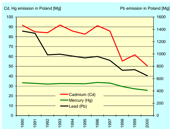
Fig. 3.8.. Trends of emissions of heavy metals: Pb, Cd, Hg [tonnes] in Poland in 1990-2000
