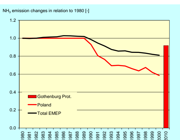
Fig. 3.6. Relative changes in NH 3 emissions in Poland and total EMEP in 1980-2000 (values related to 1980 emissions)
