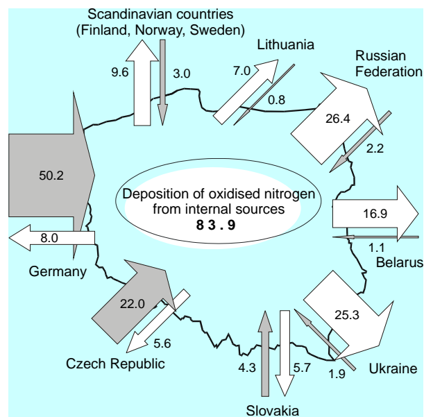
Fig. 5.2. Deposition of oxidised nitrogen compounds [10 3 t(N)/year] resulting from emission in Poland and imported to Poland, according to EMEP calculations for 1998 (based on Eulerian Acid model).
