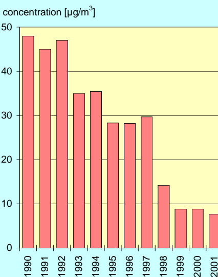
Fig. 4.2 Annual mean SO 2 concentration trends at Czerniawa station (Black Triangle) in 1990-2001
