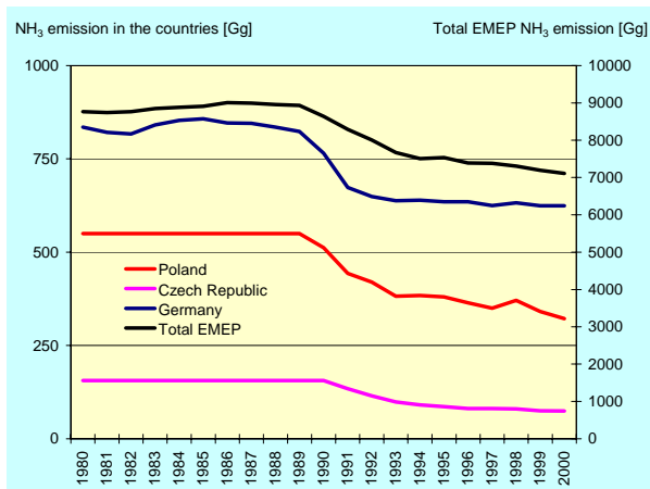
Fig. 3.5. Trends of NH 3 emissions [ktonnes] in Poland, in the selected neighbouring countries, and total EMEP in 1980-2000
