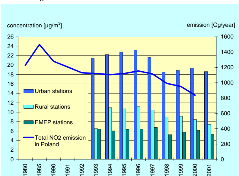
Fig. 4.5. Changes in annual mean NO 2 concentrations (averaged over the NNBS sites belonging to the groups: urban, rural, and EMEP stations-without Śnieżka) against a background of emission trends in Poland
