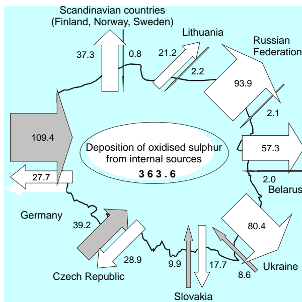
Fig. 5.1. Deposition of oxidised sulphur [10 3 t(S)/year] resulting from emission in Poland and imported to Poland, according to EMEP calculations for 1998 (based on Eulerian Acid model).
