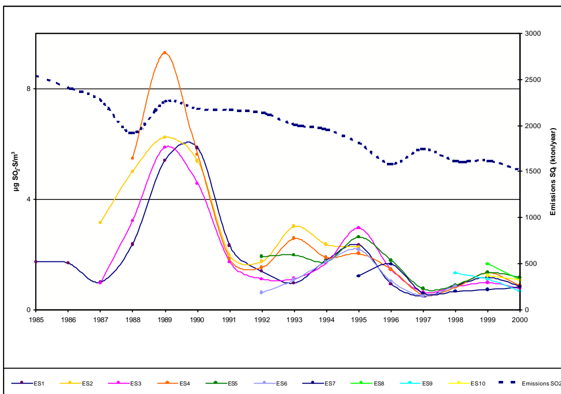
Figure 2: SO_2 annual values (1985-2000). Concentration ( \mu g S/m^3 ) vs. emission data (kton/year).
