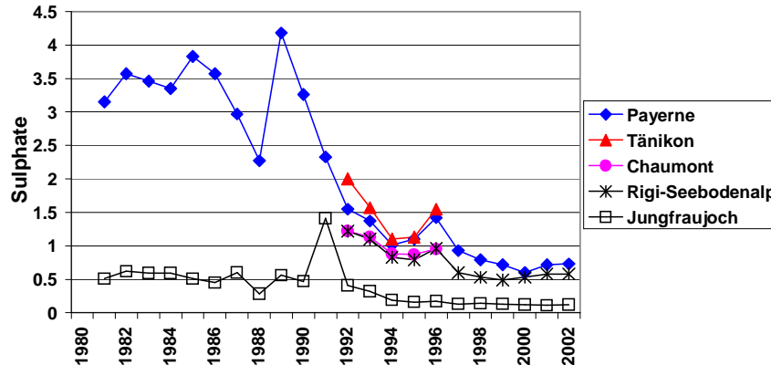
Figure 4. Annual means of particulate sulphate 1981-2002 (in µgS/m 3 ).
