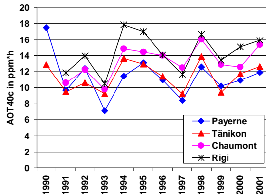
Figure 11.b AOT40 values for crops (May – July, daylight hours) in \text{ppm}^*\text{h} .
