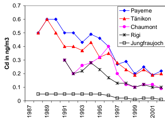
Figure 9b. Annual mean concentrations of cadmium in TSP or PM10 at Swiss monitoring sites. 1987-2002 (in ng/m³).
