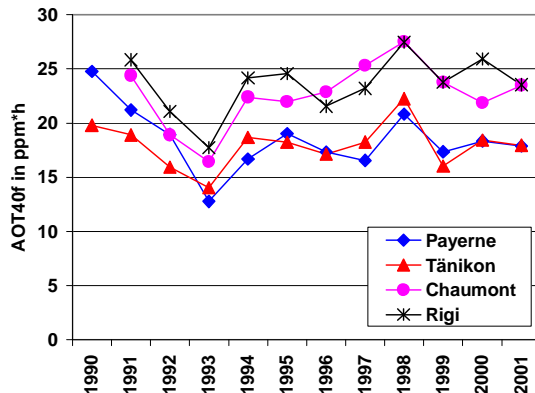
Figure 11.a AOT40 values for forests (April – September, daylight hours) in \text{ppm}^*\text{h} .
