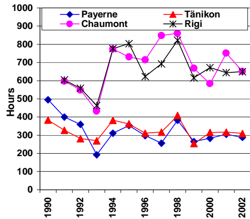
Figure 10b. Annual number of hours with an ozone concentration > 120 \mu\text{g}/\text{m}^3 .
