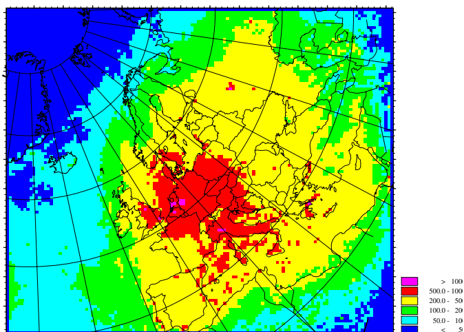
Figure 5.17: Deposition of oxidised nitrogen in EMEP model domain. Total depositions from all sources for year 2000. (Units: \text{mg}/\text{m}^2 ).
