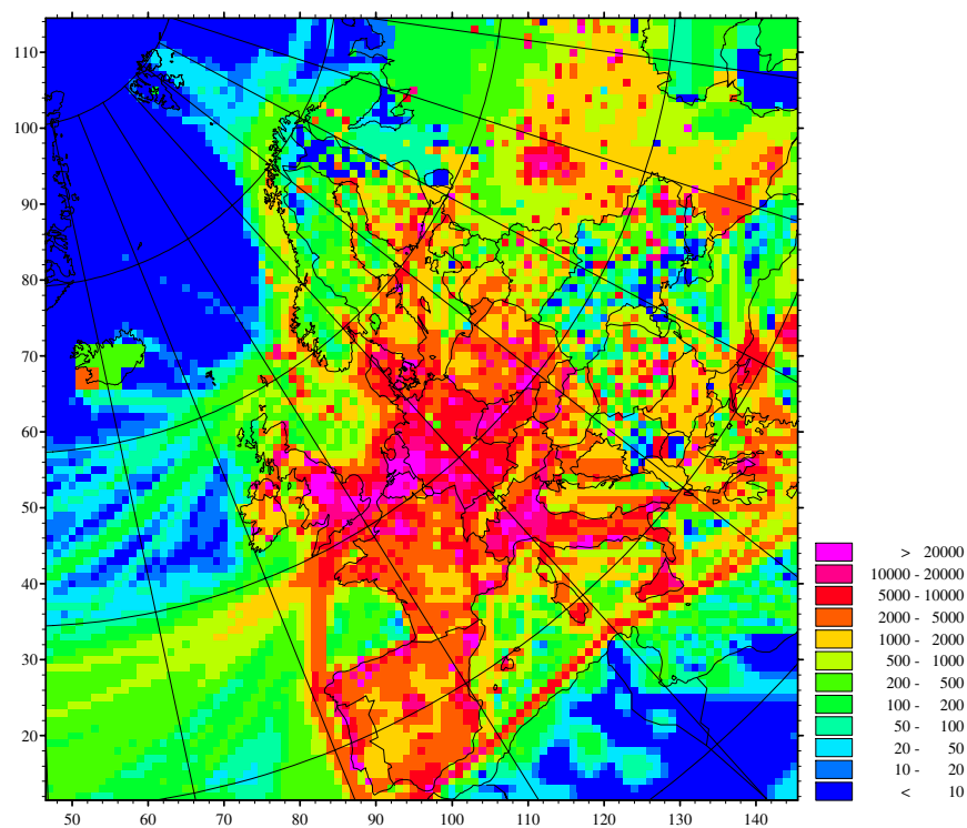
Figure 5.1: Distribution of NO x emissions from all EMEP sources as used in this study. Values for year 2000. (Units: tons/gridcell).
