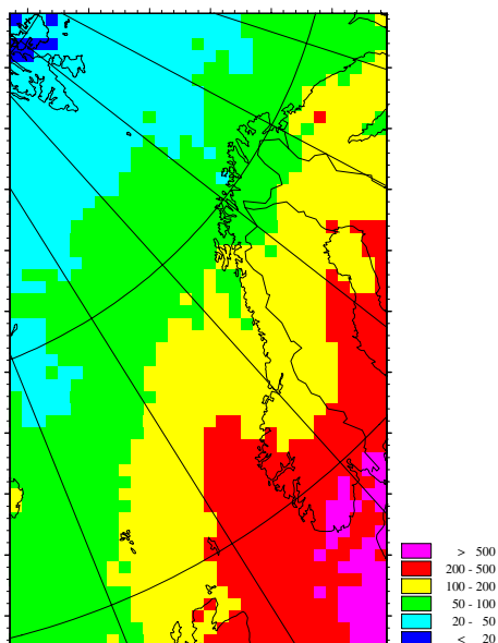
Figure 5.20: Deposition of oxidized nitrogen in the Norwegian area from all sources. Year 2000. (Units: \text{mg}/\text{m}^2 ).
