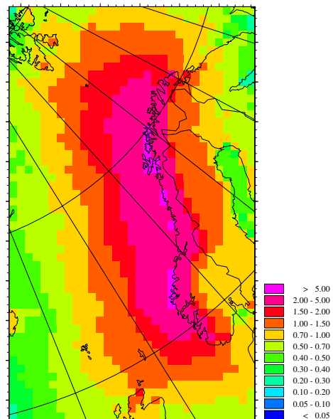
Figure 5.33: Deposition of oxidized nitrogen from Norwegian fisheries. Vessel group J: “Other purse seiner vessels”. Year 2000. (Units: mg/m 2 ).
