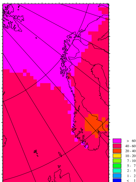
Figure 5.20: Deposition of oxidized nitrogen in the Norwegian area from all sources. Year 2000. (Units: \text{mg}/\text{m}^2 ).
