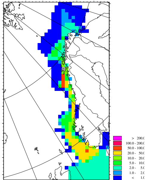
Figure 5.10: \text{NO}_x emissions from Norwegian fisheries. Vessel group E: “Shrimp freezing trawlers”. (Units: tons/gridcell).
