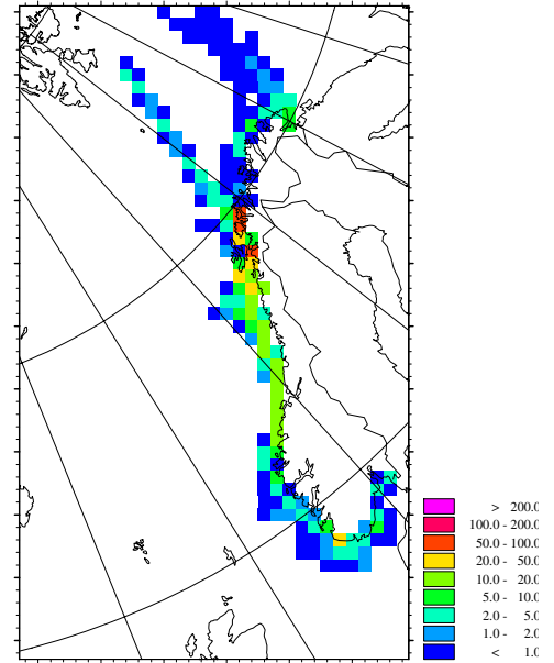
Figure 5.11: \text{NO}_x emissions from Norwegian fisheries. Vessel group F: “Other shrimp trawlers”. (Units: tons/gridcell).
