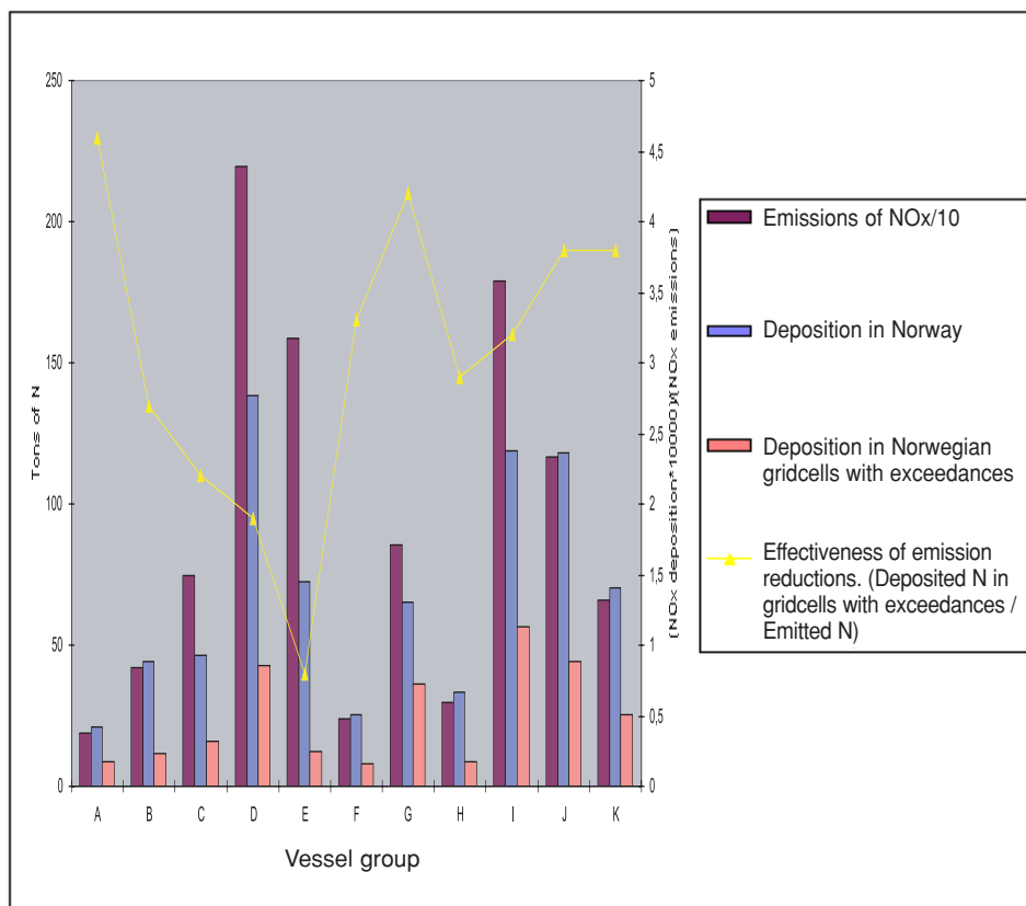
Figure 3.1: Comparison of level of NO x emissions and deposition in Norway and in Norwegian gridcells with exceedances. Note that emissions have been divided by a factor 10. Effectiveness of emission reductions are given in the right hand axis.
