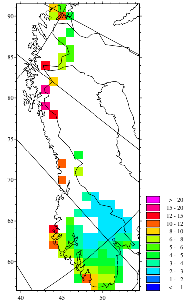
Figure 5.46: Ratio between deposition of oxidized nitrogen and emissions for vessel group F in areas with exceedance to critical load of acidity. (Units: %*100).
