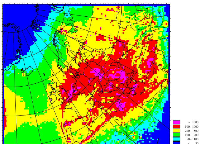
Figure 5.18: Deposition of oxidised sulphur in EMEP model domain. Total depositions from all sources for year 2000. (Units: \text{mg}/\text{m}^2 ).
