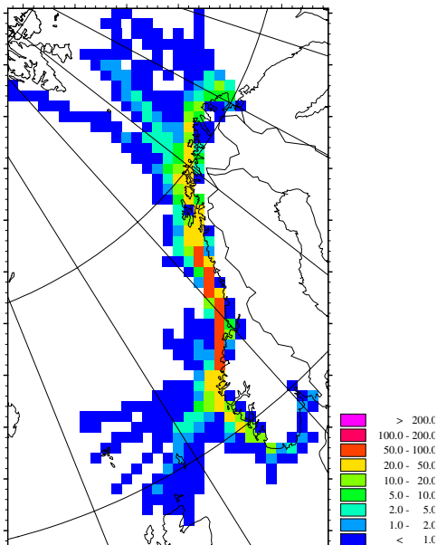
Figure 5.14: NO x emissions from Norwegian fisheries. Vessel group I: “Purse seiner with season for blue whitting”. (Units: tons/gridcell).
