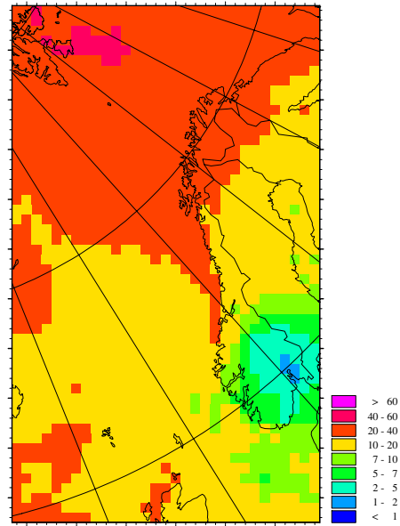
Figure 5.23: Contributions from the Norwegian fishing fleet to \text{NO}_x deposition from all Norwegian sources. Year 2000. (Units: %).
