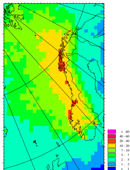
Figure 5.21: Contribution of Norwegian sources to total depositions. Year 2000. (Units: percent (%) of deposition of oxidized nitrogen).
