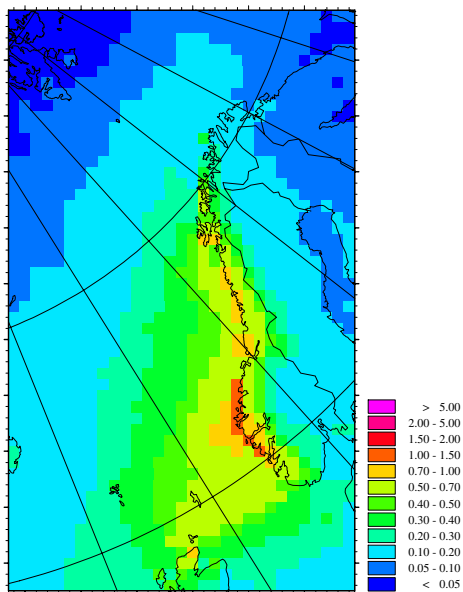
Figure 5.32: Deposition of oxidized nitrogen from Norwegian fisheries. Vessel group I: “Purse seiner with season for blue whitting”. Year 2000. (Units: mg/m 2 ).
