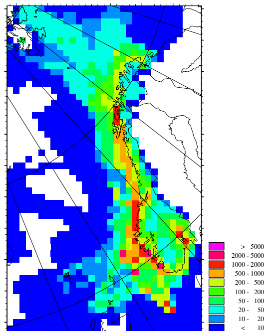
Figure 5.4: Norwegian \text{NO}_x emissions from SNAP sector 8 used in this study. (Units: tons/gridcell).
