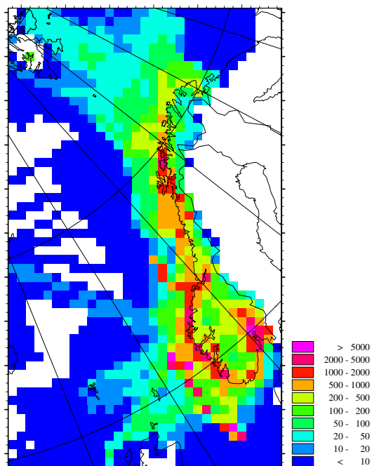
Figure 5.3: \text{NO}_x emissions from all Norwegian sources for year 2000 used in this study. (Units: tons/gridcell).
