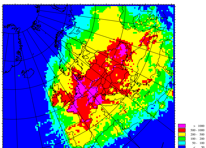
Figure 5.19: Deposition of reduced nitrogen in model domain. Total depositions from all sources for year 2000. (Units: \text{mg}/\text{m}^2 ).
