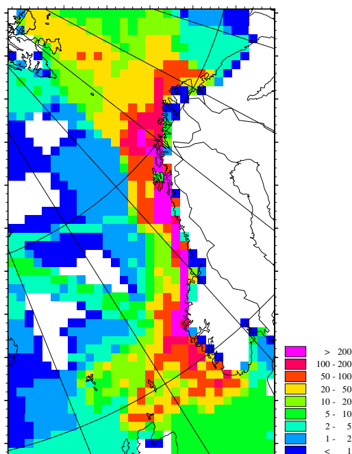
Figure 5.5: \text{NO}_x emissions from the Norwegian fishing fleet. Total emissions for all types of vessels for year 2000. Estimate by Statistics Norway. (Units: tons/gridcell).
